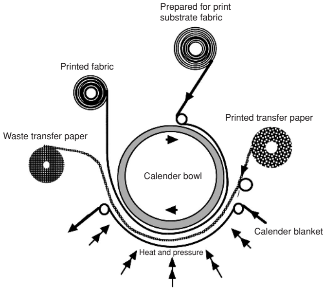
4.12 Diagram of a transfer printing machine used for polyester fabrics.
