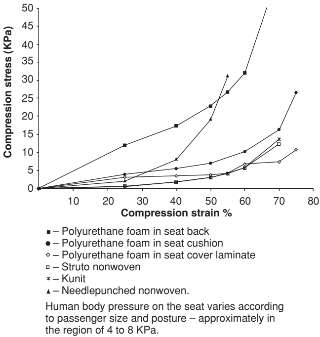
6.2 Compression stress/strain characteristics of some non-woven materials compared to polyurethane foam.
