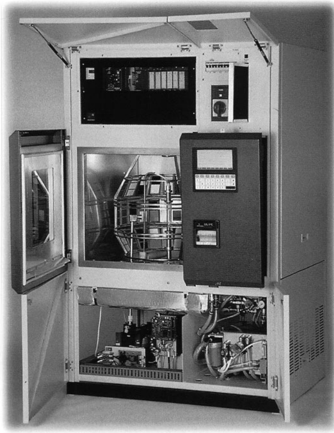
5.2 Ci4000 Weather-Ometer (Atlas Material Testing). The test samples and lamp are located in the centre of the illustration. The apparatus accurately controls the uniformity of light, temperature and humidity of the test samples. Photograph supplied by Atlas Material Testing Technology BV and reproduced with kind permission.
