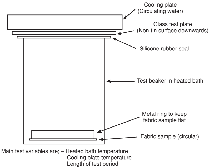
5.9 Automotive fabric fogging testing.
