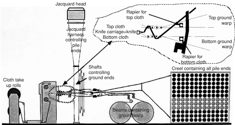
3.19 Face to face velvet jacquard weaving machine with detail inset of yarn/fabric interface. (Reproduced by kind permission of Michel Van De Wiele NV.)
