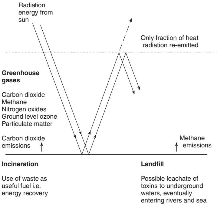
8.1 The 'greenhouse effect'.
