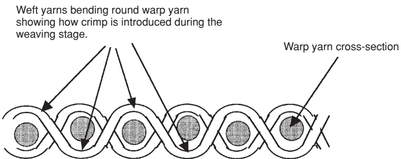
3.8 Cross-section of a plain-weave structure showing how the yarns interlace and 'crimp up'.
