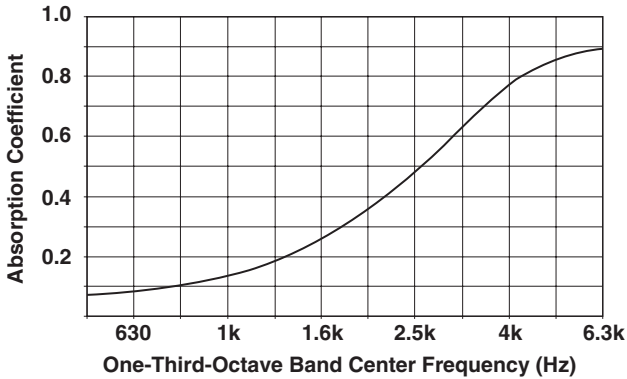
6.9 Sound Absorbing Properties of Thinsulate™ Acoustic Insulation. Sound Absorbing properties of Thinsulate™ Acoustical Insulation material AU1220, measured according to ASTM E1050, Dual Microphone Impedance Tube Method measuring Normal Incidence Sound. Thinsulate™ acoustic insulation provides especially good results at the high frequencies which are particularly unpleasant to the human ear. Diagram produced by 3M Company and reproduced with kind permission of 3M Deutschland GmbH.
