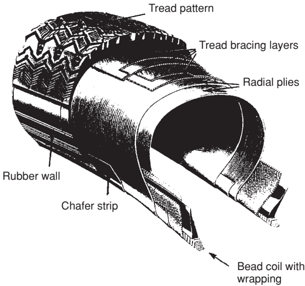
7.3 Textile components of a car tyre. Simple diagram showing the main textile components. From an illustration provided by the British Rubber Manufacturers' Association and reproduced with kind permission.
