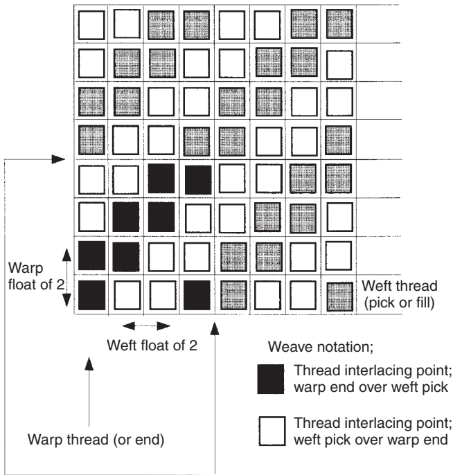
3.11 Point paper notation of 2 \times 2 twill weave.
