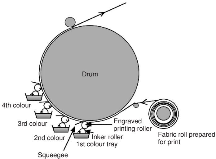
4.9 Simplified diagram of roller printing by engraved copper roller, showing set up for a 4 colour printed design.
