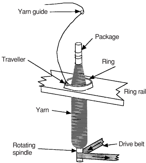
3.1 Basic elements of ring spinning.
