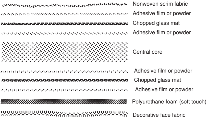
6.5 Typical multilayer headliner construction. The central core is semi-rigid polyurethane foam, resinated shoddy waste fibres or some other material. Heat is applied to the assembly in a flat-bed laminator to join all the components together. The material is then cut into lengths, heat is applied and the headliner is press-moulded to the required shape. During the latter process the assembly is compressed to about one-third of its original thickness. The adhesive film or powder permeates through the chopped glass mat and consolidates it. The chopped glass mat contributes to rigidity and acoustic insulation.
