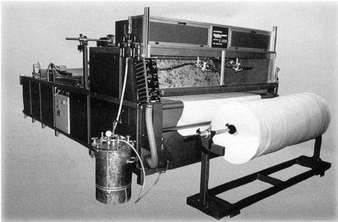
4.23 Machtex Multi-purpose spray adhesive laminating and coating machine, Type CMW-3. Reproduced with kind permission of Mach Tex Holland BV.
