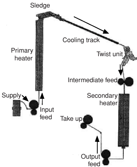
3.2 False twist texturing. (Reproduced by kind permission of Rieter-Scragg Ltd.)
